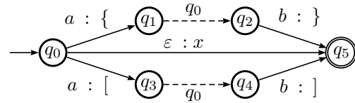
Figure 1: Example of RTNSO. Labels of the form x : y represent an input : output pair (e.g.: a : \{ for transition (\delta(q_0, a, \{) = (q_1, \lambda) ). Dashed transitions represent a call to the state specified by the label (e.g.: transition (\delta(q_1, \varepsilon, \varepsilon) = (q_2, q_0) ).
